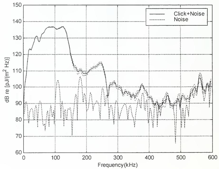
Figure 4.9 Eight Dolphin Clicks And Corresponding Average Energy Flux Spectral Density With 1/4" Filter Present ( \pm 1\sigma shown as dot-dash line)
